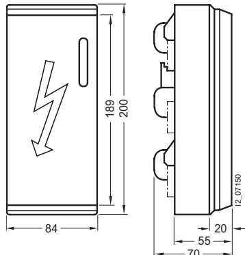
8US19 21-1AA00
