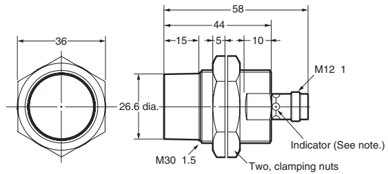
E2A-M30KN18-M1-□□/E2A-S30KN18-M1-□
