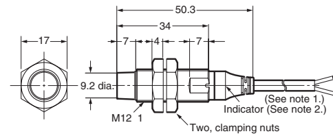
E2A-M12KN05-WP-□□/E2A-S12KN05-WP-□
