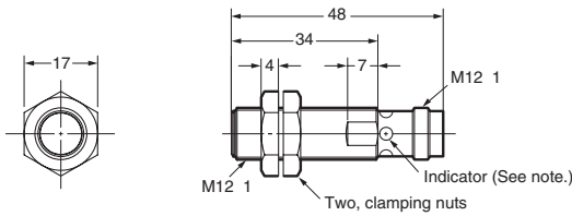
E2A-M12KS02-M1-□□/E2A-S12KS02-M1-□
