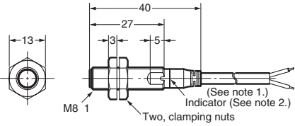
E2A-S08KS01-WP-□□
