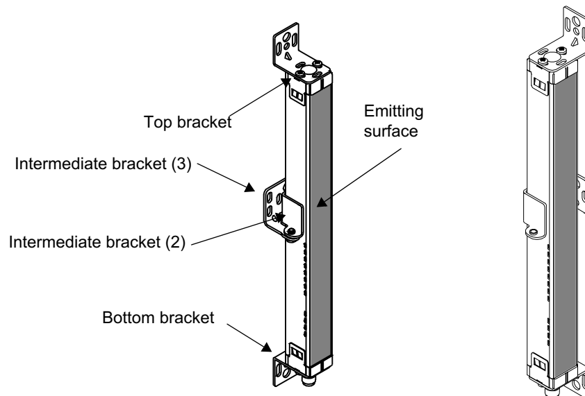
[Rear mounting]
