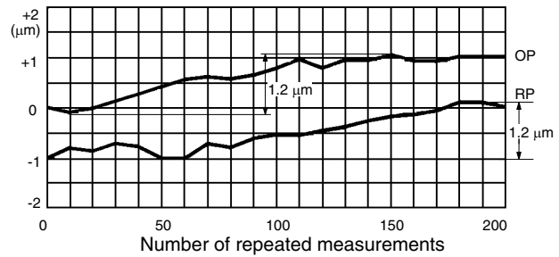
M16 Type (Contact/Solid-state Output) With Repeat Accuracy of 3 μm max. D5A-7□□□ Series
