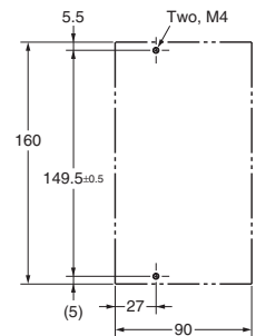
Mounting dimensions
