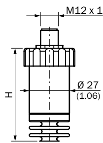
Housing with circular connector M12 x 1, IP 67
