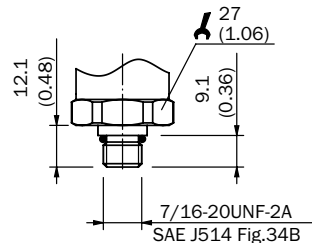
7/16" -20 UNF
