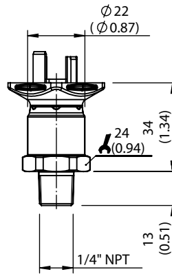
Process connection 1/4" NPT with connection for L-connector according to DIN EN 175301-803 A
