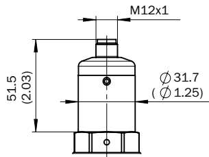
Housing (standard temperature range -40 °C ... 100 °C), M12 x 1, IP 67
