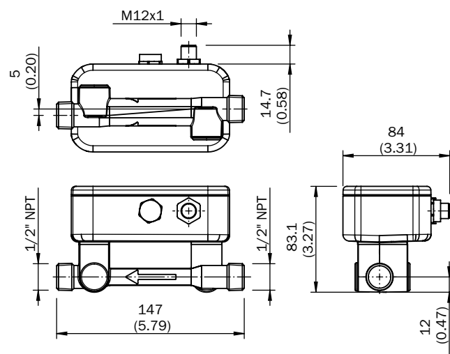
NW 10, 1/2" NPT
