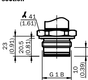
G 1 B without cooling section
