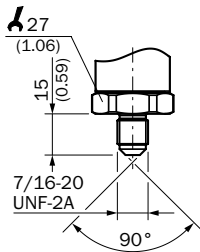
7/16" -20 UNF
