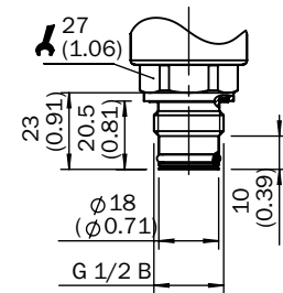
G 1/2 B flush-mounted
