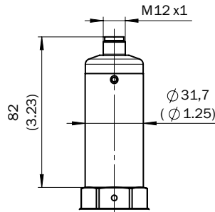
Housing (enhanced temperature range -40 °C ... 150 °C)
