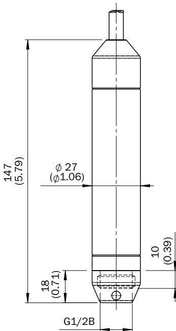
Enhanced version with FEP cable (Immersion depth up to 100 m)
