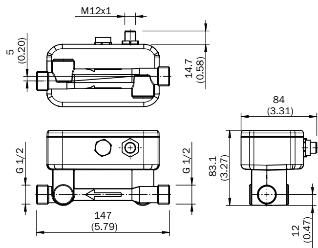
NW 10, G 1/2
