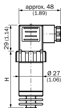
Housing with L-connector (DIN 175301-803 A), IP 65
