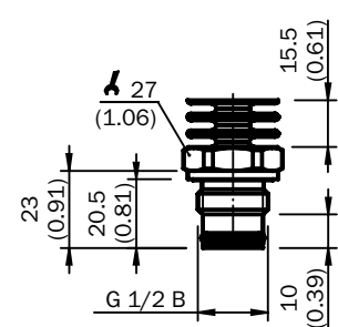
G 1/2 B with cooling section
