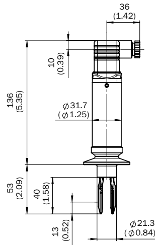
Tri-Clamp 1", 2"
