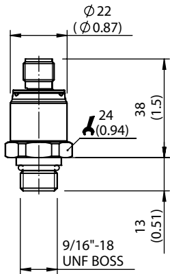
Process connection 9/16"-18 UNF SAE #4 J514 male with O-ring Boss (FKM) with round connector M12 x 1, 4-pin
