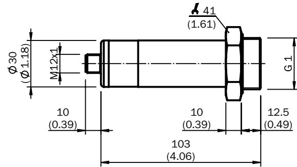
UP56-211/ 212/ 213 all-metal
