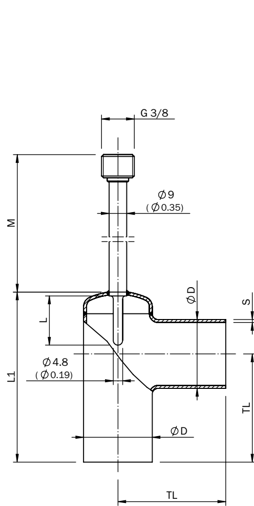
Protection tube with process connection
