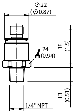
Process connection 1/4" NPT with round connector M12 x 1, 4-pin
