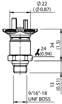
Process connection 9/16"-18 UNF SAE #4 J514 male with O-ring Boss (FKM) with connection for L-connector according to DIN EN 175301-803 A
