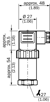
G 1/4 female
