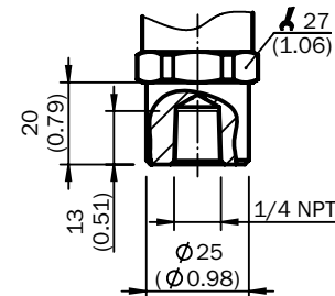
1/4" NPT female
