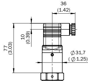
Housing (standard temperature range -40 °C... 100 °C), DIN 43650 incl. plug angled/IP 65
