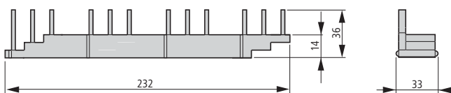
B3.1/4-PKZ4
