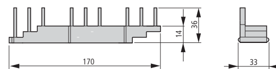
B3.1/3-PKZ4
