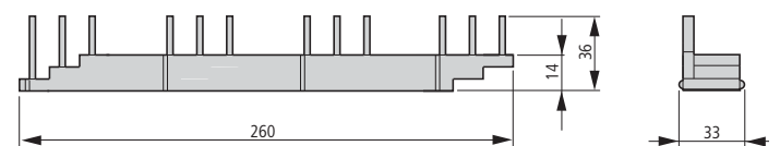
B3.2/4-PKZ4
