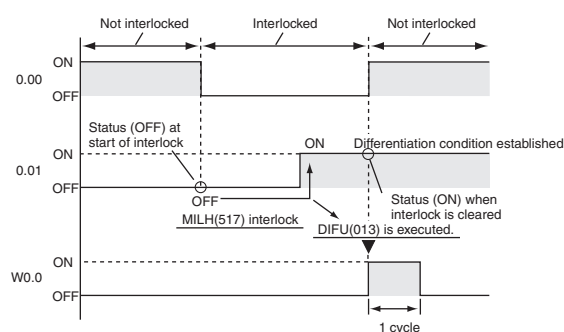
Timing chart
