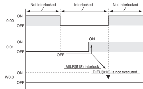
Timing chart
