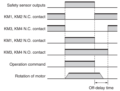
Timing chart
