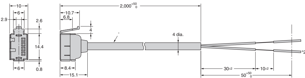
* E3X-CN21: 4-dia. vinyl-insulated round cable with 4 conductors (Conductor cross section: 0.2 mm², Insulator diameter: 1.1 mm)
